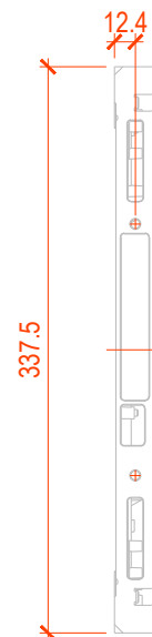
Infinity S Side view
