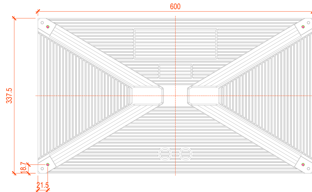
Infinity S Rear view
